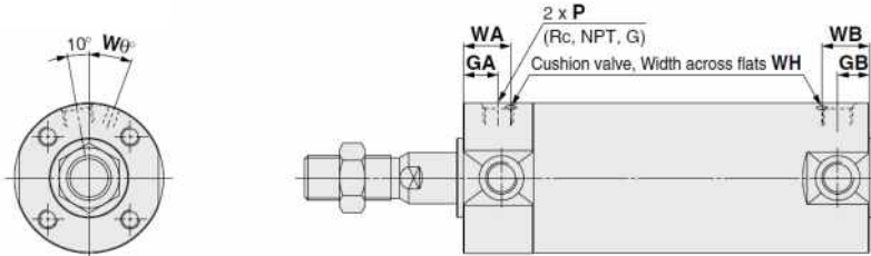
Basic (Without trunnion mounting female thread): CG1ZN
