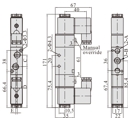
4V220(Terminal)
