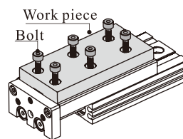
Top Mounting
